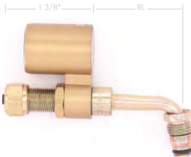
PT GAUGE on valve (side view)
